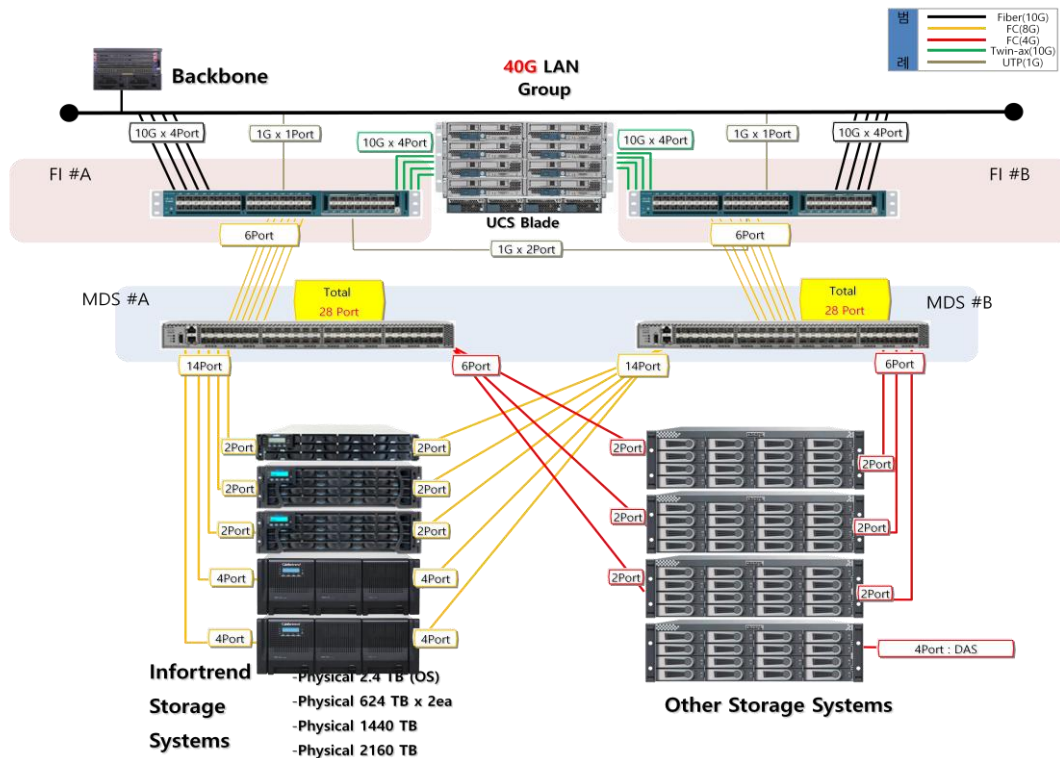
System Diagram
